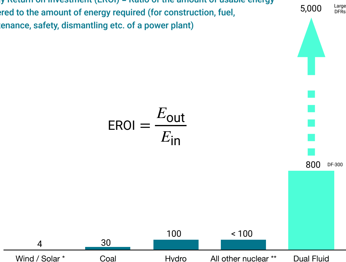
Figure 5: Energy return of current energy sources vs. Dual Fluid
