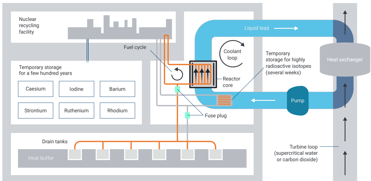
Figure 2: Schematic diagram of DF1500 power plant with on-site recycling. The fuel is permanently processed so that all fissionable material is returned to the reactor. Residuals are stored for about 300 years.
