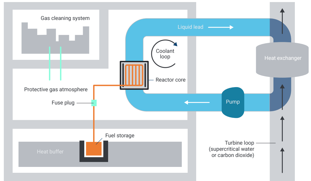
Figure 1: Schematic diagram of modular power plant DF300. The fuel is delivered to the power station in a sealed cartridge. It is then heated and pumped into the reactor core where it generates heat for about 25 years. At the end of the burning cycle, the spent fuel is transported to a Dual Fluid recycling facility.
