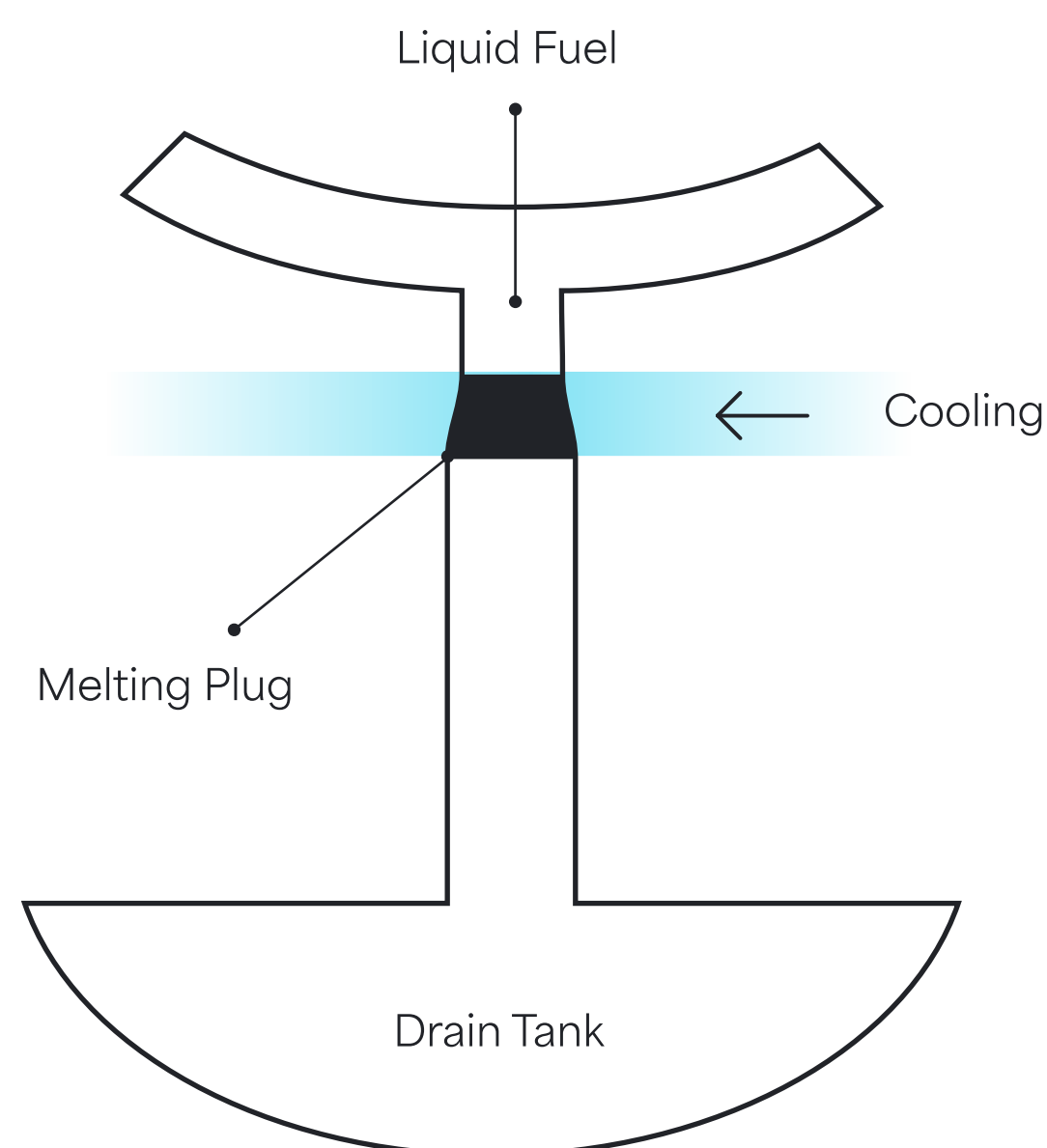
Figure 6: Sketch of the fuse plug. As soon as the cooling fails or is no longer sufficient, the fuel drains downwards into safe tanks and the chain reactions stops immediately
